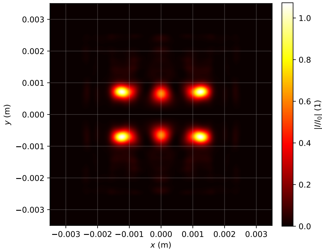
Intensity profile I(x, y, z = 2.627)/I_0 , P_{in}=6.0P_{cr} , artificial time
